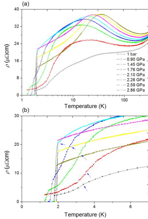
Fig. 2. (a) Temperature dependence of the in-plane electrical resistivity \rho of a 0.45 % Hg-doped CeRhIn 5 under pressure on a semilogarithmic scale. (b) The in-plane electrical resistivity of a 0.45 % Hg-doped CeRhIn 5 is magnified near the phase-transition temperatures. Blue arrows mark the antiferromagnetic transition temperatures.
